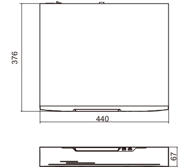
Figure 2-1 Dimensions (Unit:mm)
