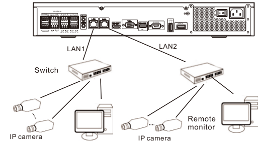
Figure 4-2 Topology of the NVR
