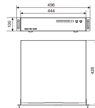
Figure 2-1 Dimensions (Unit:mm)
