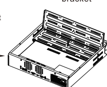
Figure 3-2 Lift the upper bracket
