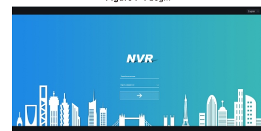
Figure 7-1 Login
