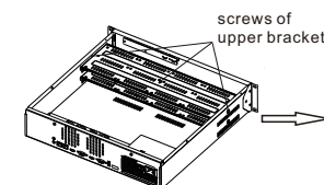
Figure 3-1 Unscrew the screws
